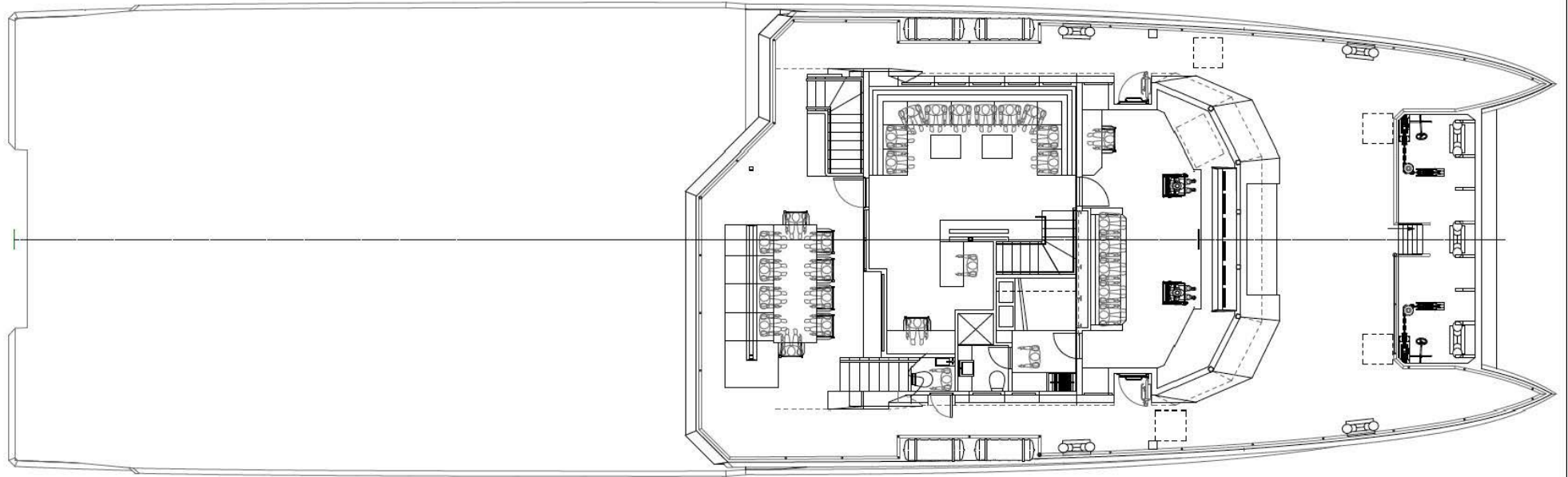
BRIDGE DECK
